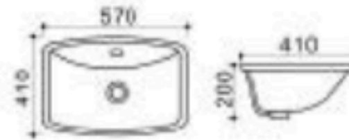
UP-017 Size: 570X410X200mm
