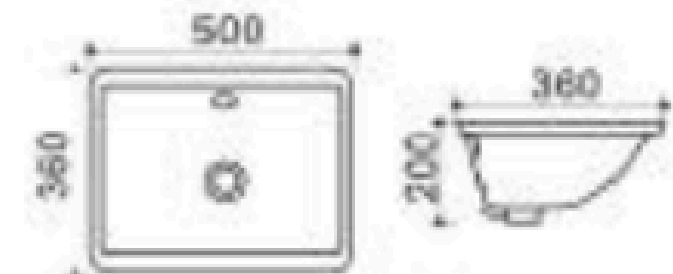
UP-012 Size: 500X360X200mm
