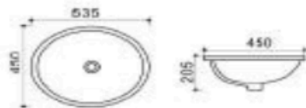
UP-018 Size: 535X450X205mm
