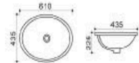
UP-019 Size: 610X435X225mm
